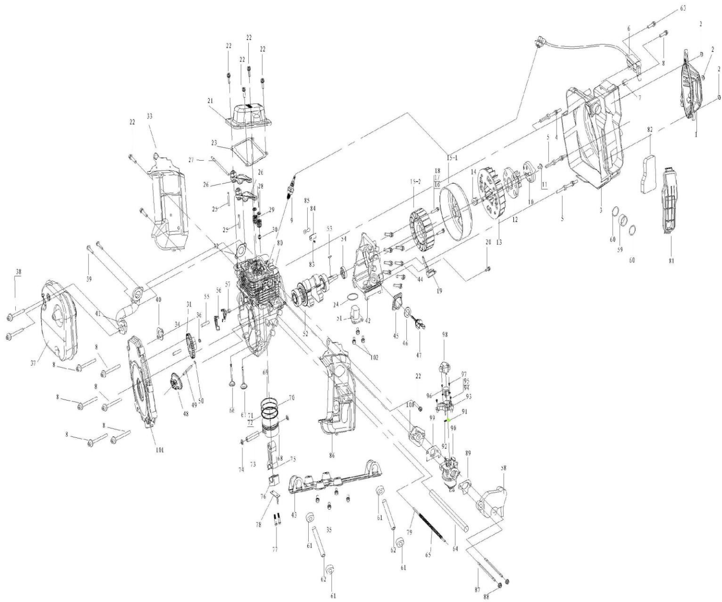
1200iEngine parts Component diagram
